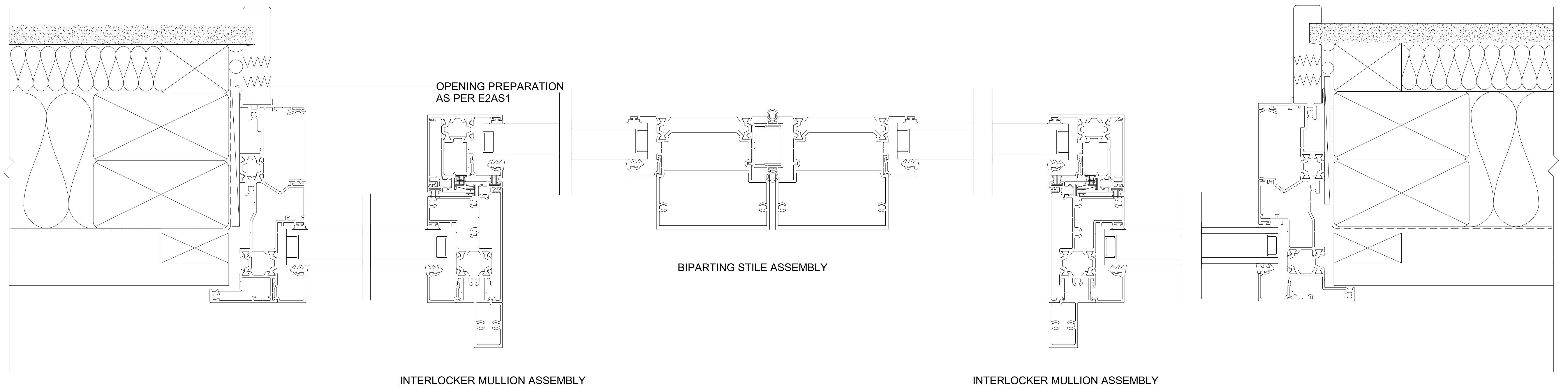
INTERLOCKER MULLION ASSEMBLY
